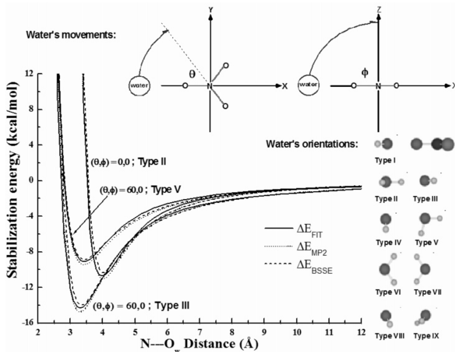
Figure 1. Comparison of the interaction energies obtained from the MP2 calculations with and without basis set superposition error (BSSE) correction, \Delta E_{\text{MP2}} and \Delta E_{\text{BSSE}} , and from the fitted potential function, \Delta E_{\text{FIT}} , using the parameters given in Table 2 for some values of \theta and \phi .
