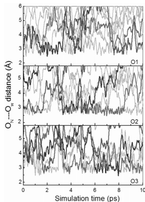
Figure 11. Time dependence of \text{O}_N-\text{O}_w distances, selecting only for the first 10 ps of the HF/MM simulation.
