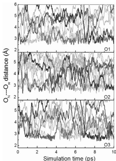
Figure 12. Time dependence of \text{O}_N\text{---O}_w distances, selecting only for the first 10 ps of the B3LYP/MM simulation.
