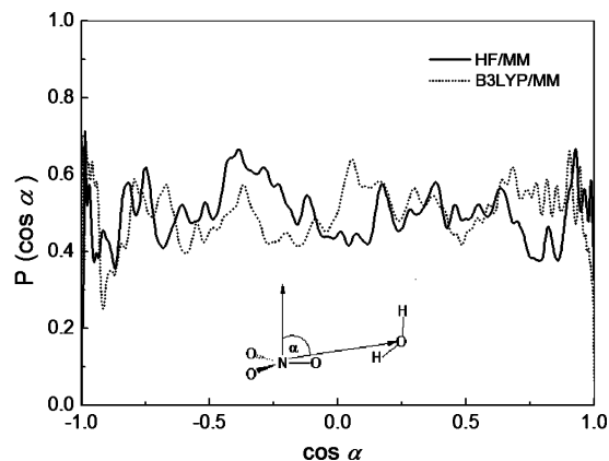
Figure 3. Distributions of the angle \alpha between the vector perpendicular to the \text{NO}_3^- plane and the vector along the \text{N}\cdots\text{O}_w distance, calculated within the first minimum of \text{N}\cdots\text{O}_w RDFs.
